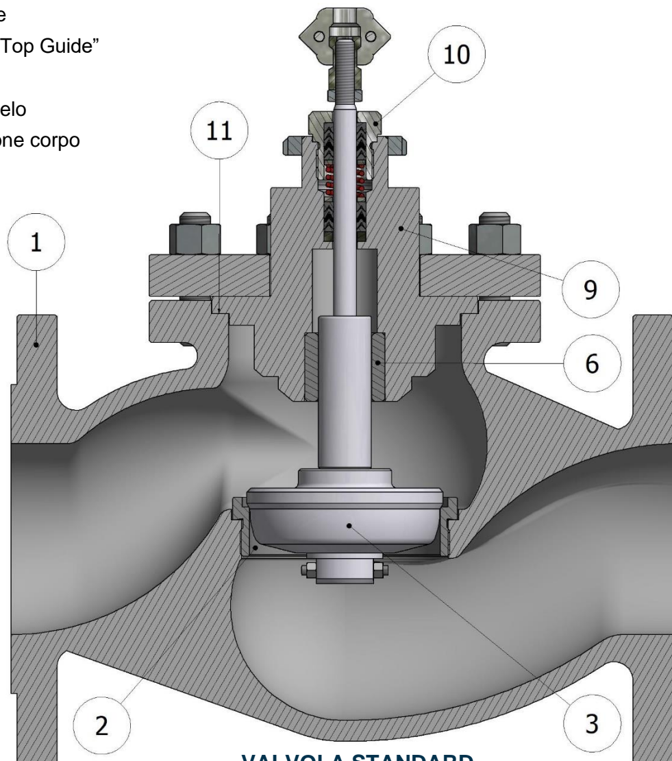
VALVOLA STANDARD
