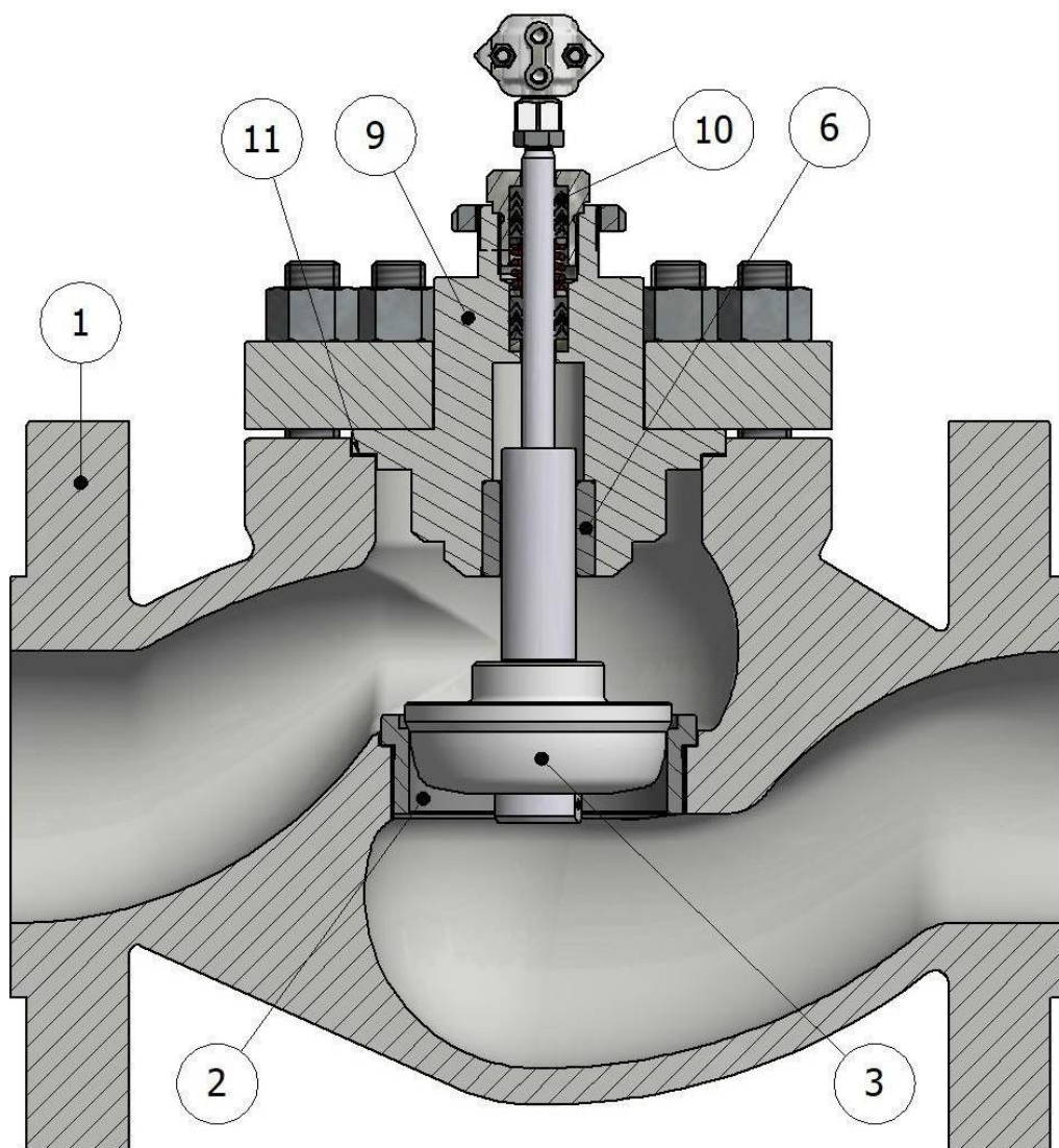
VALVOLA STANDARD
